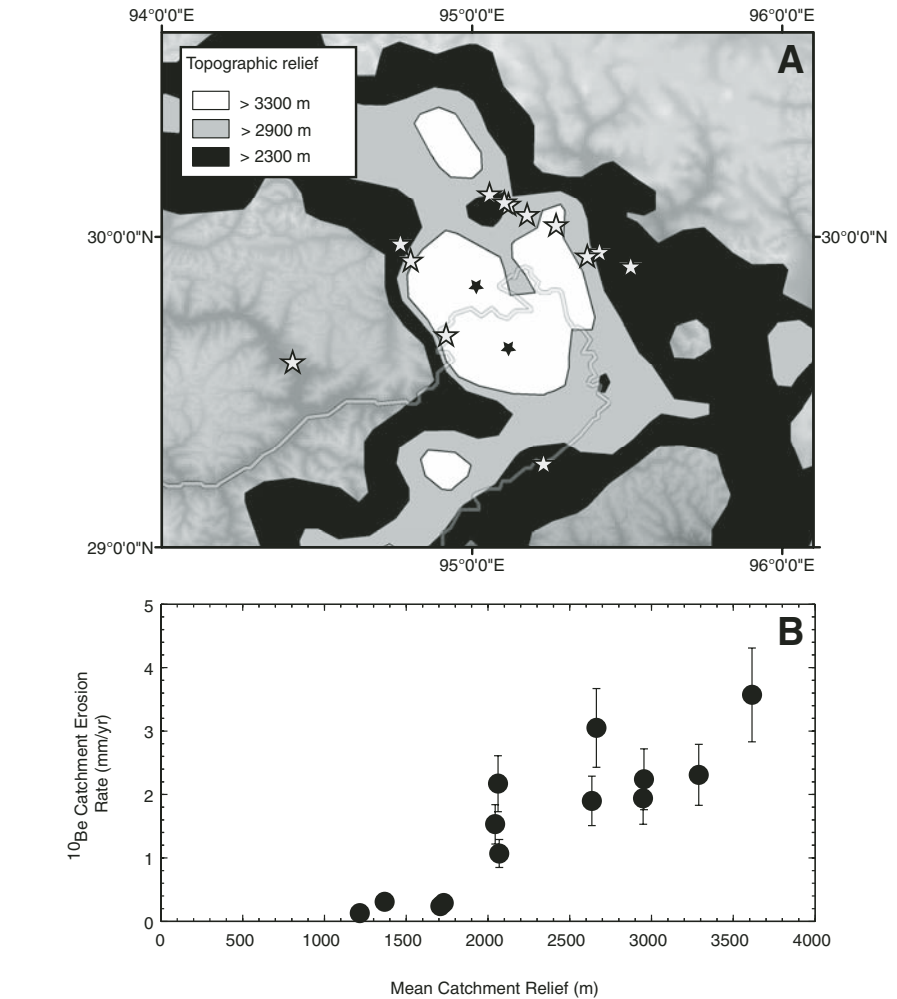
Figure 4. (A) Patterns in topographic relief in the vicinity of the Namche Barwa–Gyala Peri massif. Areas with no data coverage are those with relief <2300 m. Gray stars denote the locations of sediment samples taken for ^{10}\text{Be} analysis. Black stars show the locations of Namche Barwa and Gyala Peri. (B) ^{10}\text{Be} basin-averaged erosion rate vs. mean topographic relief for sampled catchments.
